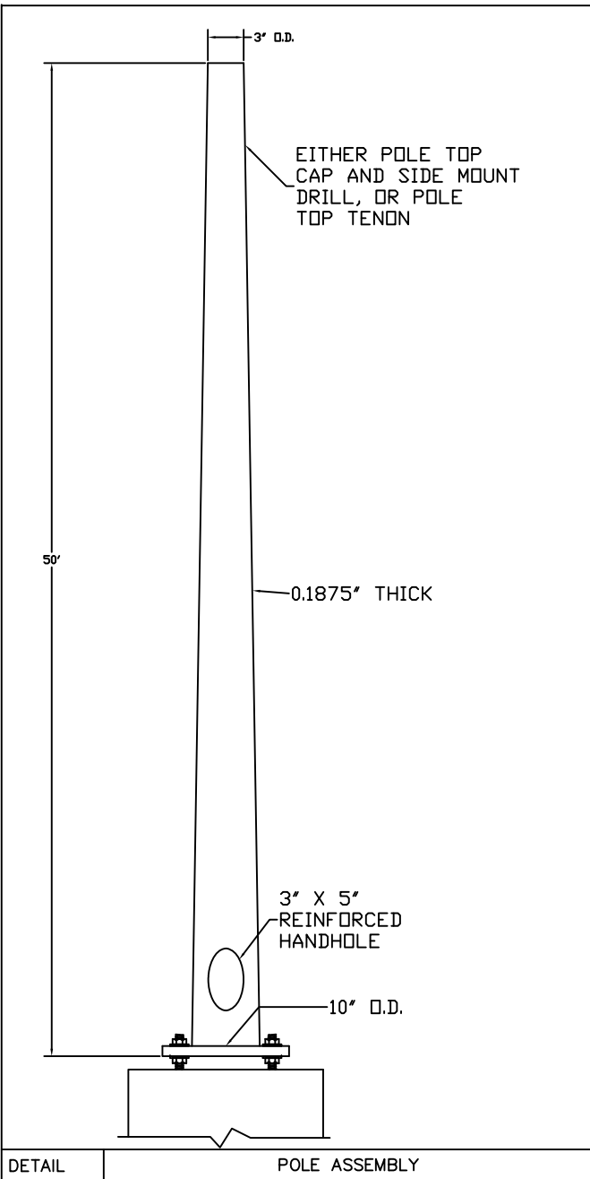
DETAIL POLE ASSEMBLY
